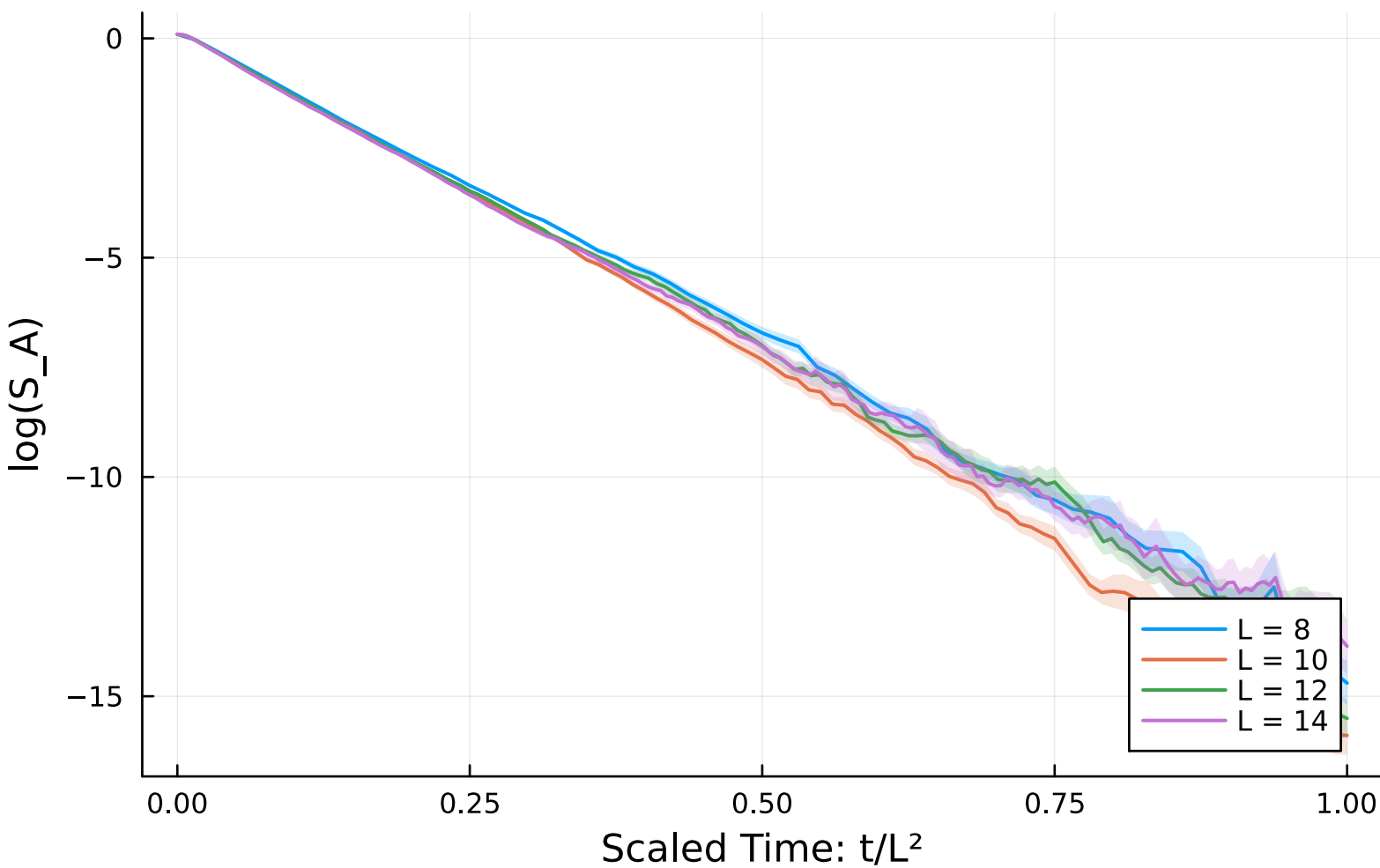
Scaled Log Entropy Evolution ( p = 0.500000 )
